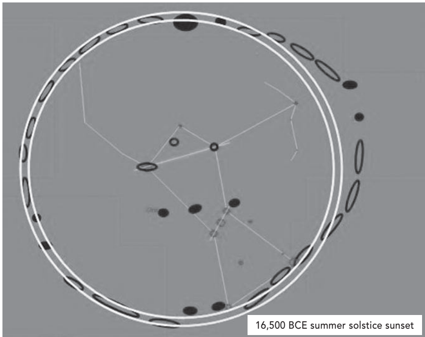
Figure 4.4. Orion's head and shoulders matching the Calendar Circle stones at altitude, azimuth, and date
