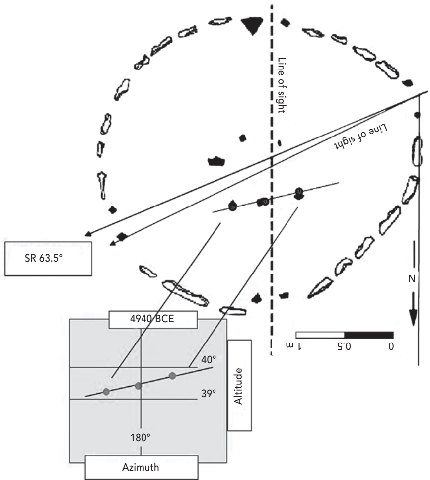
Figure 4.3. Diagram of Orion's belt matching Calendar Circle stones at altitude, azimuth, and date.
