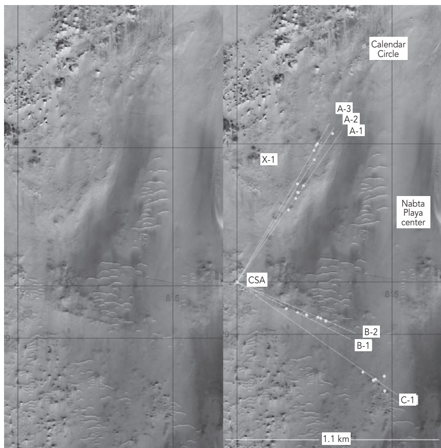
Figure 4.7. Satellite image of the area of Nabta Playa containing the megalith alignments. Left, satellite image with black gridlines for measuring; right, the megalith alignments and the Calendar Circle appear labeled, but the circle stones are too small to be seen in the satellite image.
