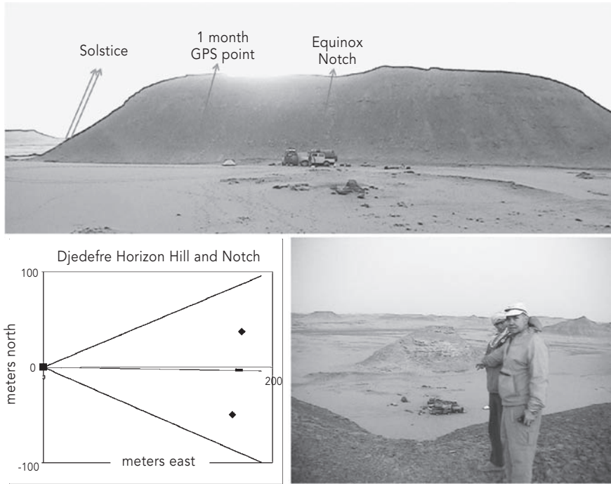
Figure 4.13. Sunrise over Horizon Hill at Djedefre sun temple, April 2008. Top: the rising azimuths at equinox over the notch in the hill and the approximate solstice rising azimuth. Lower right: Brophy and Bauval standing, before sunrise, at Horizon Hill notch and pointing to the east, facing the Djedefre cartouche. Lower left: the three GPS points taken at the top of Horizon Hill—at the notch and two central hilltop locations—the azimuths to sunrise over the notch from the Djedefre cartouche, and the solstice sunrises.
