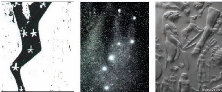
Figure 4.8. Left, ancient Egyptian depiction of the Big Dipper as the Bull's Thigh; middle, photo of constellation; right, constellation as sculpted on the Denderah zodiac ceiling
